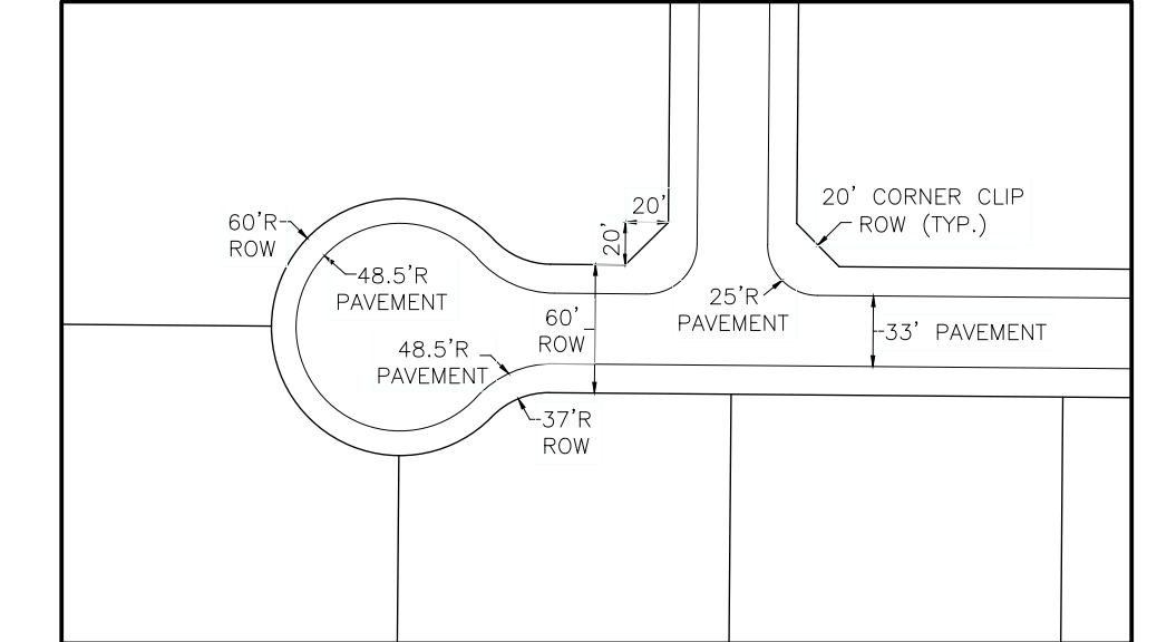
TYPICAL INTERSECTION/CUL-DE-SAC DETAIL NOT TO SCALE
